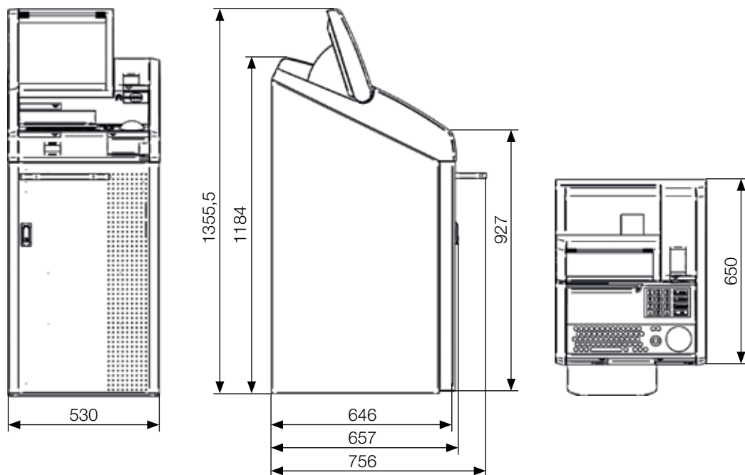
KePlus K6 Kontoserviceterminal
